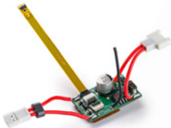
O201c1 oXigen chip in-car controller
